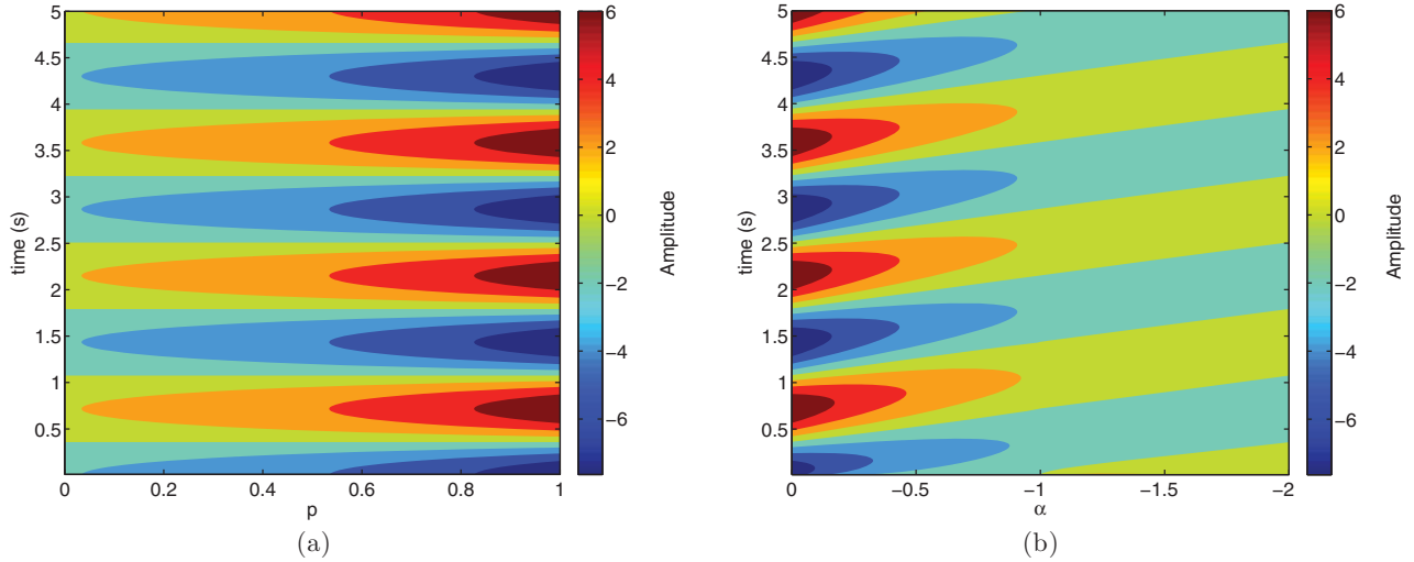
Figure 3. Forward path signal propagation for the 1-link planar pendulum: (a) \vartheta_1 ; (b) \psi_1 . The pendulum parameters are l_1 = 1 , m_1 = 1 , r_1 = 0.5 , and the initial conditions are \theta = 0.4 , \dot{\theta} = 0 .
