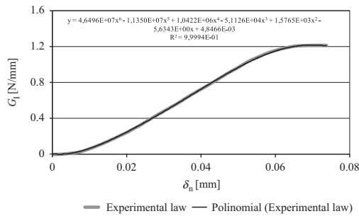
Fig. 9. Experimental G_I - \delta_n law for one specimen and polynomial fitting.
