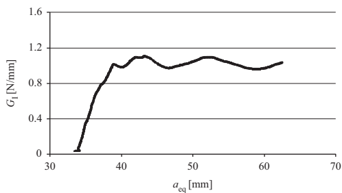
Fig. 5. Evolution of G_I with a_{eq} for a test specimen with h=3 mm.
