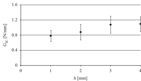
Fig. 10. Average values and deviation of G_{IC} as a function of h by the J -integral.
