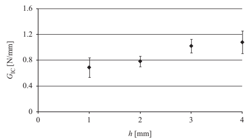
Fig. 6. Average values and deviation of G_{IC} as a function of h by the CBBM.
