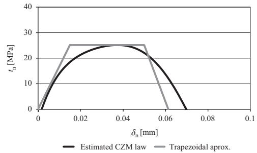
Fig. 11. Estimated t_n - \delta_n law for one test specimen and approximation.
