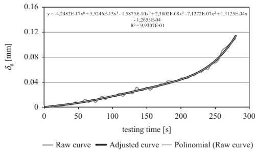
Fig. 8. Plot of \delta_n -testing time for a specimen with h=4 mm: raw curve, polynomial approximation and adjusted polynomial curve.
