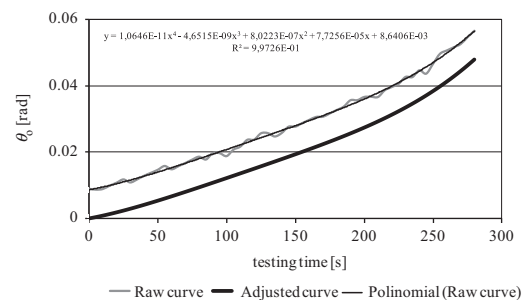
Fig. 7. Plot of \theta_0 -testing time for a specimen with h=4 mm: raw curve, polynomial approximation and adjusted polynomial curve.
