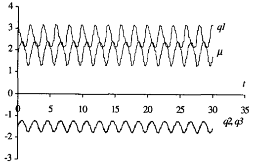
Fig. 3. The 3R-robot joint positions versus time using the OLM method for r = 1 , \rho = 0.5 .
