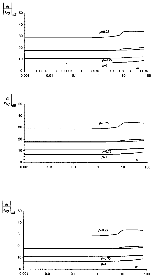
Fig. 14. Frequency response of the CLP method for the 3R robot and r = 2 and \rho \in \{0.10, 0.25, 0.50, 0.75, 1.00\}
