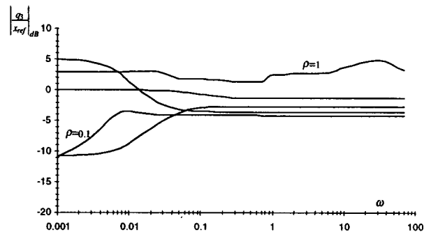
Fig. 13. Frequency response of the CLP method for the 3R robot and r = 2 and \rho \in \{0.10, 0.25, 0.50, 0.75, 1.00\}
