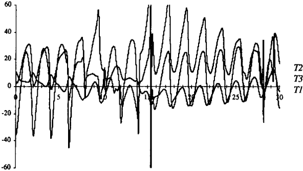
Fig. 4. The 3R-robot joint torques versus time using the CLP method ( r = 1, \rho = 0.5 ). The joint 1 maximum torque is T_1 = 158.1 \text{ Nm} at t = 15.3 \text{ sec} . The joint 2 maximum torque is T_2 = 67.6 \text{ Nm} at t = 15.3 \text{ sec} . The joint 3 maximum torque is T_3 = 14.7 \text{ Nm} at t = 11.5 \text{ sec} .
