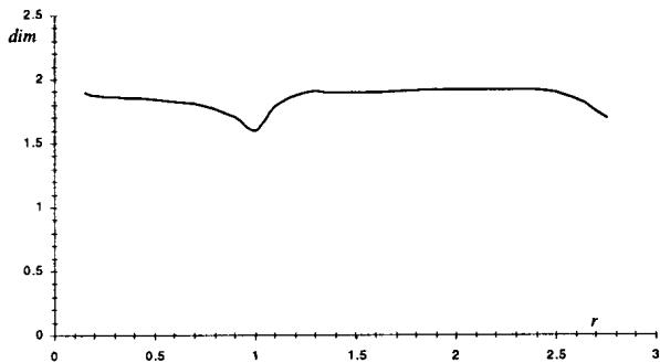
Fig. 10. Fractal dimension dim of the kinematic phase-plane versus the radial distance r for the 3R ( \rho=0.1 ) with de CLP method.
