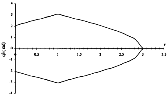
Fig. 12. Most probable robot joint positions vs the radial distance r .
