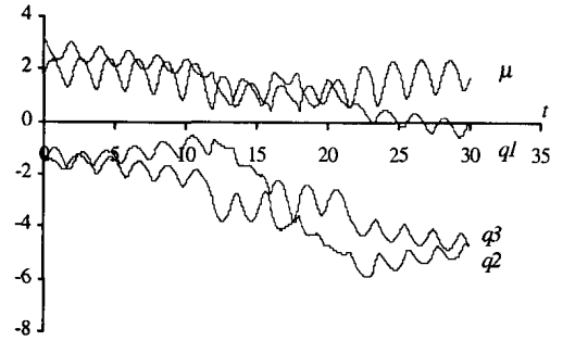
Fig. 2. The 3R-robot joint positions versus time using the CLP method for r = 1 , \rho = 0.5 .
