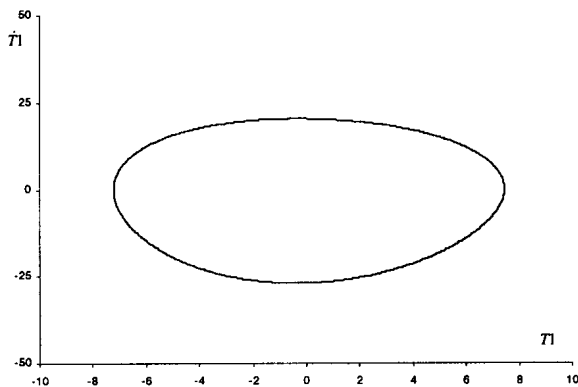
Fig. 9. Phase plane \{T_1, \dot{T}_1\} trajectory for the 3R-robot torque 1 under OLM method at r=1 , \rho=0.1 , dim=1 .
