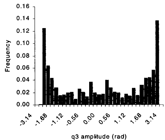
Fig. 11. Histogram for the 3R robot joint positions, with final gripper position: (x, y) = (\sqrt{2}, \sqrt{2}) .
