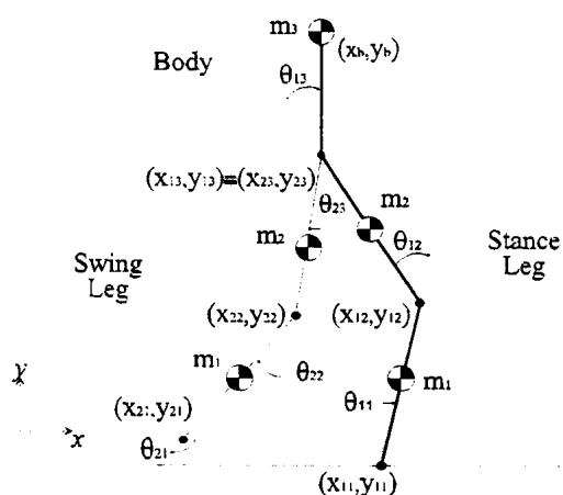
Fig. 1 - Planar biped model.
