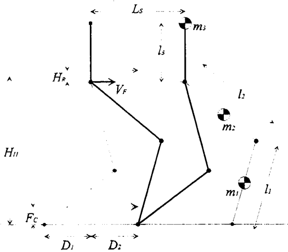
Fig. 2 - Locomotion variables.
