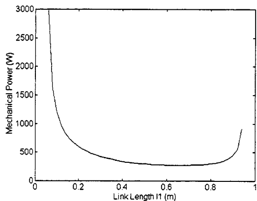
Fig. 11 - Performance index P_m vs link length l_1 .
