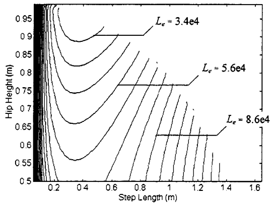
Fig. 4 - Mean power lost L_e vs H_H and L_S .
