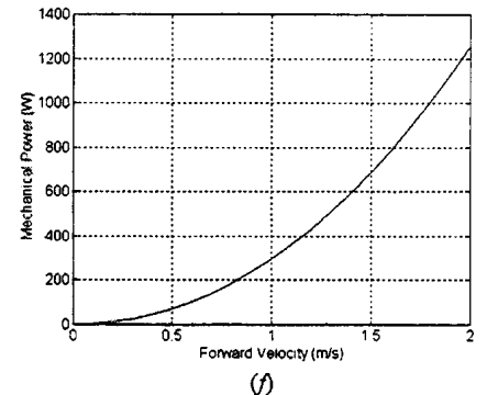
Fig. 6 - Contour plots of the absolute power P_m at the individual joints: (a) stance ankle, (b) stance knee, (c) swing hip, (d) swing knee; (e) Optimal (L_S, H_H) locus vs forward velocity V_F , (f) Absolute power vs forward velocity V_F .
