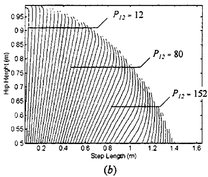
Fig. 6 - Contour plots of the absolute power P_m at the individual joints: (a) stance ankle, (b) stance knee, (c) swing hip, (d) swing knee; (e) Optimal (L_S, H_H) locus vs forward velocity V_F , (f) Absolute power vs forward velocity V_F .
