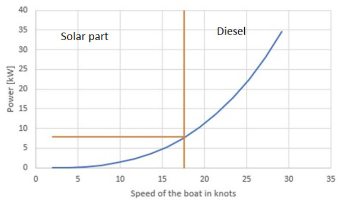
Figure 2. Power distribution
