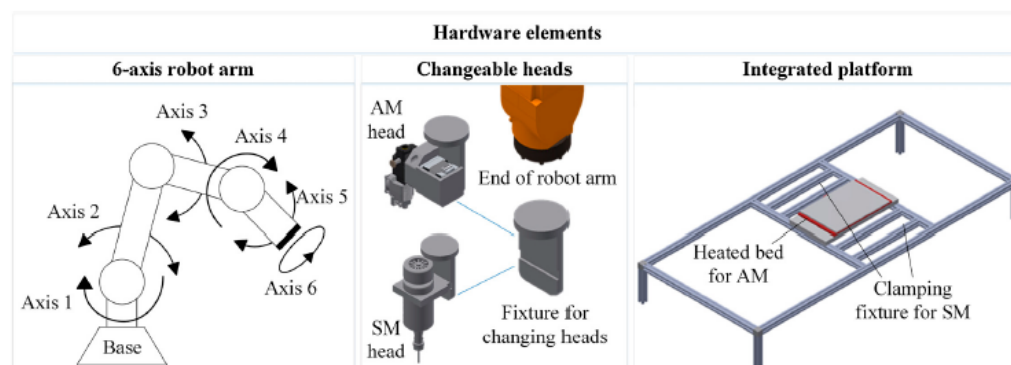
Figure 10. Configuration used in the study for the hybrid additive–subtractive manufacturing process. Reproduced from [105], 2018, Elsevier.
