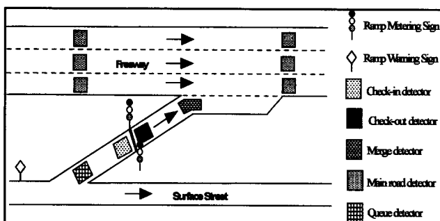
Fig. 3 – Ramp metering layout [16]
