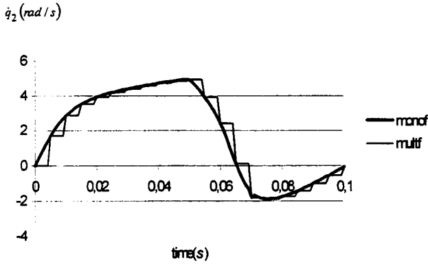
Fig. 4: Time evolution of the joint 2 velocity ( l_1 = l_2 = 1.0 m) Monofrequency: f_a = f_v = f_p = 10^3 Hz Multifrequency: f_a = 500 Hz, f_v = 200 Hz, f_p = 10^2 Hz
