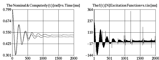
Fig. 4. The trajectory tracking and the excitation function generated by the “alternative” controller
