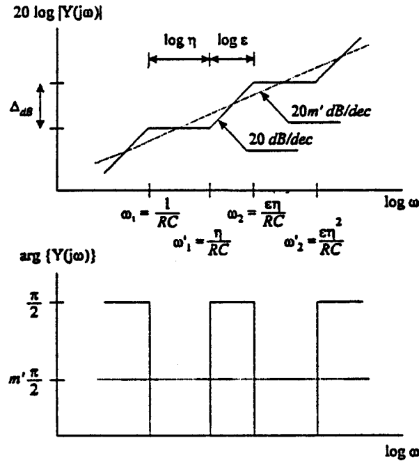
Fig. 2 Asymptotic Bode diagrams of amplitude and phase of Y(j\omega) .
