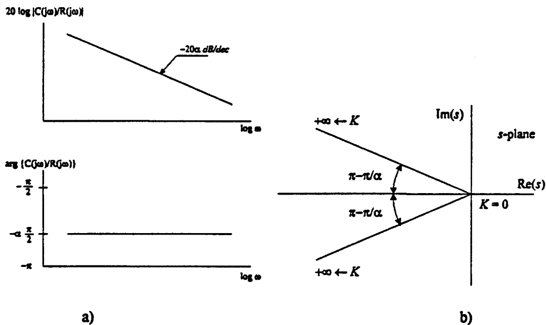
Fig. 4 Stability analysis for a feedback control system of fractional order 1 < \alpha < 2 .
