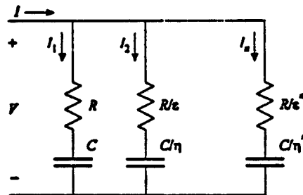
Fig. 1 Electrical circuit with recursive association of lumped resistance and capacitance elements.
