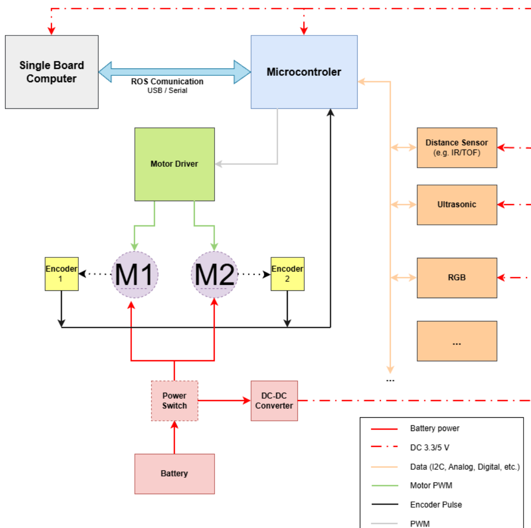
Figure 5. Generic hardware–software architecture (adapted from RobotCraft [4]).
