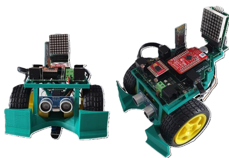
(a) Mobile robotic platform integrating a PSoC. Reproduced from Suarez et al. (2023) , Figure 7, under the Creative Commons Attribution Licence (CC BY).
