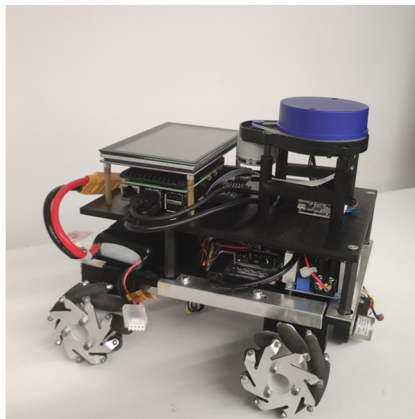
Figure 4. 5dpo platform adapted from competition to educational use. Image provided by Moreira .
