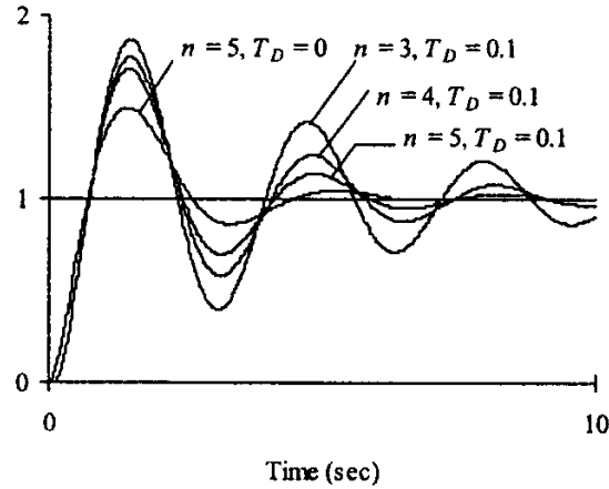
Fig. 9 Time response for G(s) = e^{-sT_D} / Ms^2 with M = 1 , T_D = 0 and T_D = 0.1 , under the control of a Letnikov-based approximation of D^{1/2} with truncation orders of n = 3, 4 and 5 . The sampling period is T = 0.1 \text{ sec} and the controller gain is K = 10\sqrt{2/T} .
