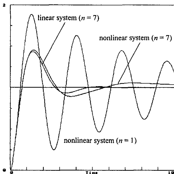
Fig. 14 System response, with deadzone, for a 7^{\text{th}} order series approximation to D^{1/2}
