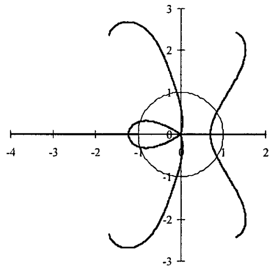
Fig. 8 Root-locus for G(s) = e^{-sT_D} / Ms^2 with M = 1 and T_D = 0 under the control of a 5 th order series approximation of D^{1/2} algorithm based on the approach of a) Letnikov b) Tustin c) Simpson.
