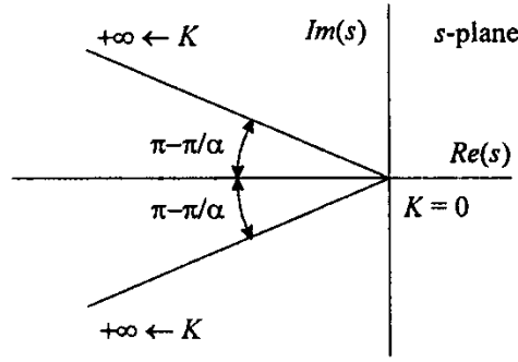
Fig. 5 Root locus for a feedback control system of fractional order 1 < \alpha < 2 .
