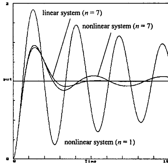
Fig. 15 System response, with hysteresis, for a 7 th order series approximation to D^{1/2} .
