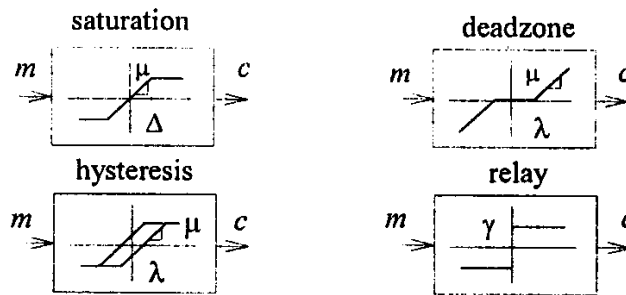
Fig. 11 Nonlinear phenomena at the actuator: saturation ( \mu = 1, \Delta = 1 ), deadzone ( \mu = 1, \lambda = 0.1 ), hysteresis ( \mu = 1, \lambda = 0.1 ) and relay ( \gamma = 1 ).
