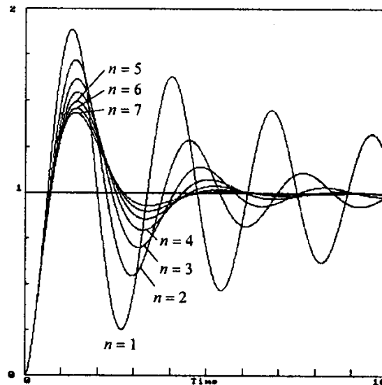
Fig. 12 Linear system response for a n^{\text{th}} order series approximation to D^{1/2} .
