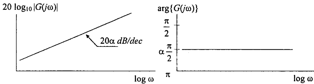
Fig. 4 Open-loop Bode diagrams of amplitude and phase for a system of fractional order 1 < \alpha < 2 .
