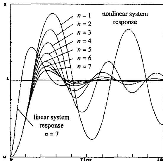
Fig. 13 System response, with saturation, for a n^{\text{th}} order series approximation to D^{1/2}
