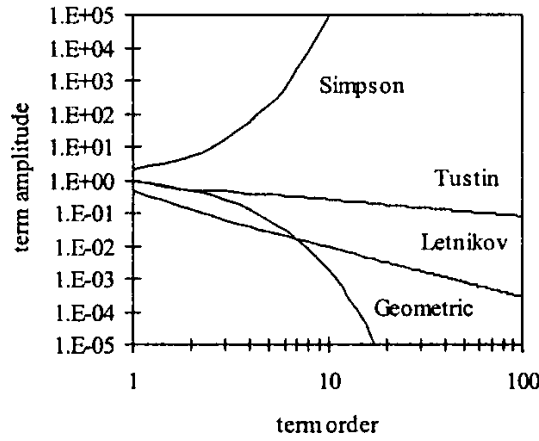
Fig. 6 Amplitude of the Taylor series coefficients versus the term order when approximating the D^{1/2} with the Letnikov, Tustin and Simpson algorithms.
