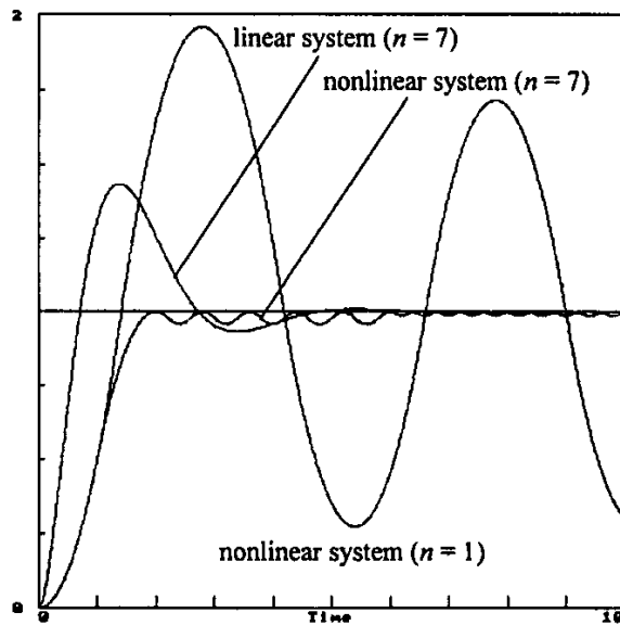
Fig. 16 System response, with relay, for a 7 th order series approximation to D^{1/2} .
