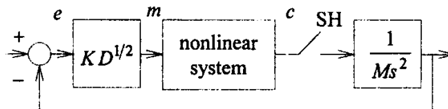
Fig. 10 A D^{1/2} controller for a system with a mass M and a nonlinear actuator.
