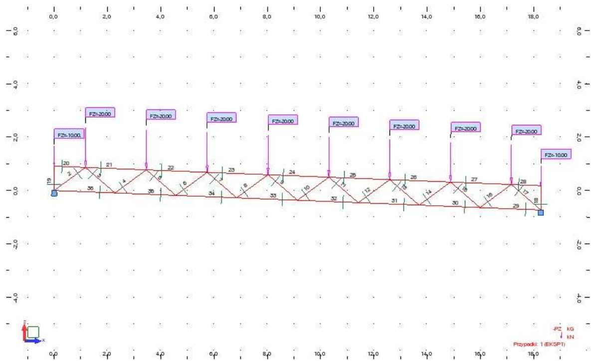
Figure 2.5.1 Truss with changes shape and IPN cross-sections.
