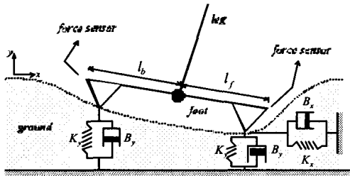
Figure 2: Constraint environment model.
