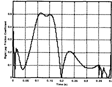
Figure 7: Friction coefficient to avoid sliding (right leg).
