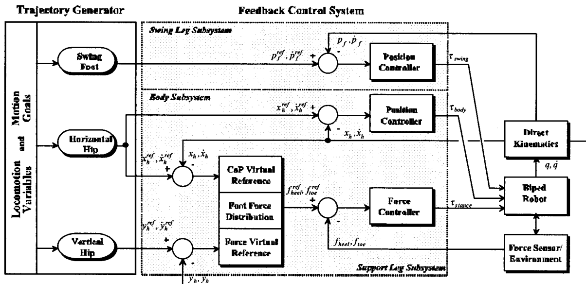
Figure 3: Goal-Oriented Force Interaction Control (GO-FIC).
