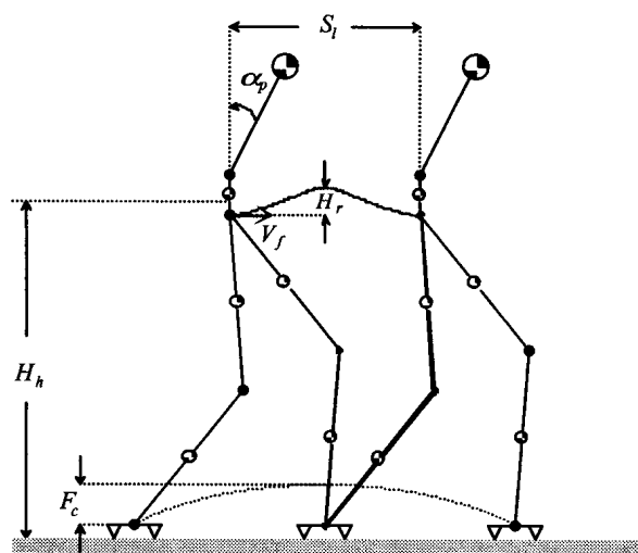
Figure 1: Planar biped model.
