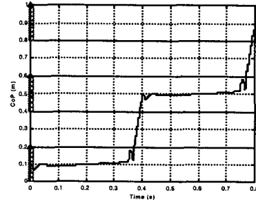
Figure 6: CoP trajectory during one complete cycle.
