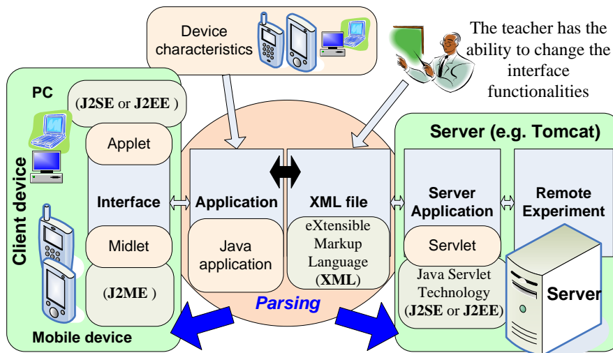
Figure 8: Proposed architecture to implement a ME scenario
