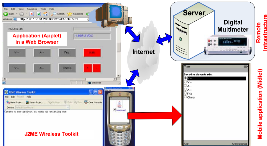
Figure 9: Architecture to control the digital multimeter
