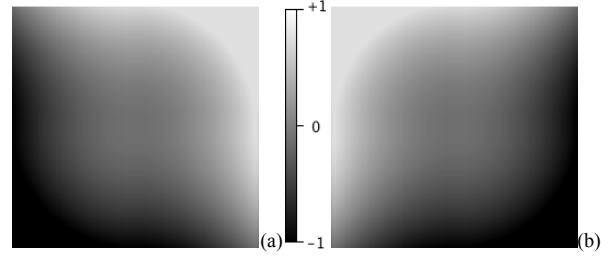
Figure 4. (a) and (b) respectively represent the left and right wheel speed mapping as a function of the x and y positions of the joystick – algorithm A with attenuation.
