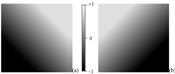
Figure 3. (a) and (b) respectively represent the left and right wheel speed mapping as a function of the x and y positions of the joystick – algorithm A.
