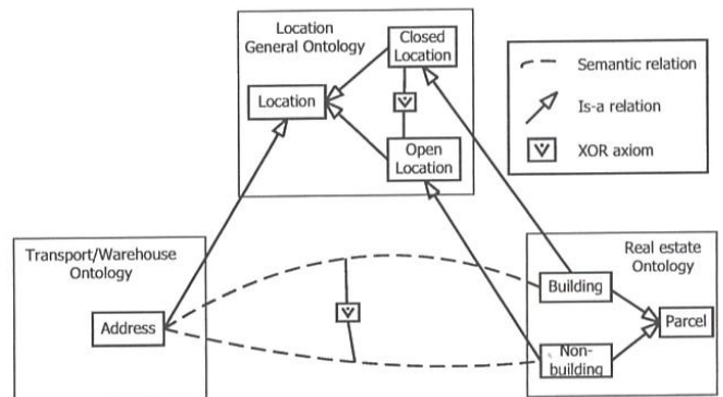
Fig. 5. Common General Ontology used
