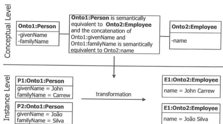
Fig. 1. Informal representation of ontology mapping
