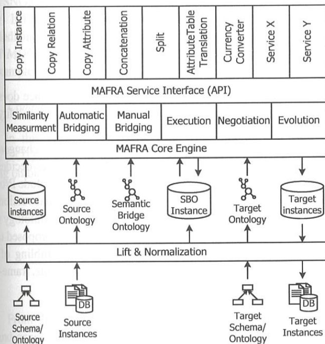
Fig. 3. Service-Oriented Architecture
