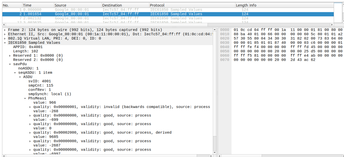
FIGURE 6.6: SV packet with bad quality sample counter with value 115.
