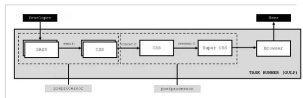
Figure 4. The CSS workflow with the two CSS processor types.
