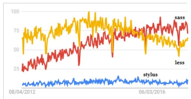
Figure 2. Interest over time on SASS, LESS and Stylus preprocessors—Google Trends.
