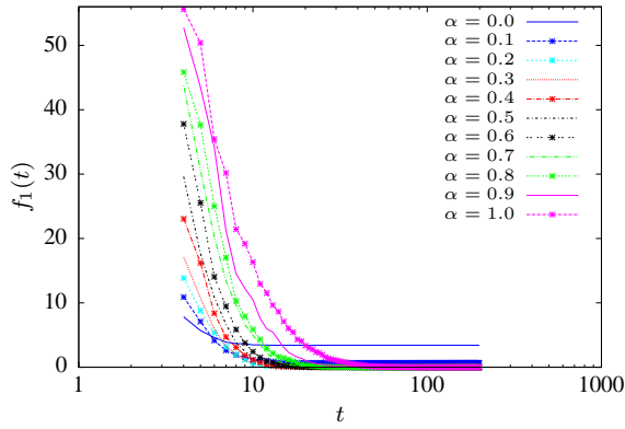
Figure 1: Evolution of the Rosenbrock's function for \alpha = \{0, \dots, 1\}
