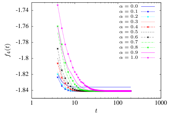
Figure 4: Evolution of the Michalewicz's function for \alpha = \{0, \dots, 1\}
