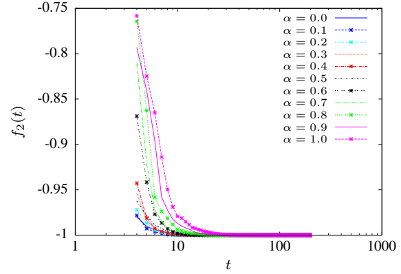
Figure 2: Evolution of the Drop wave function for \alpha = \{0, \dots, 1\}
