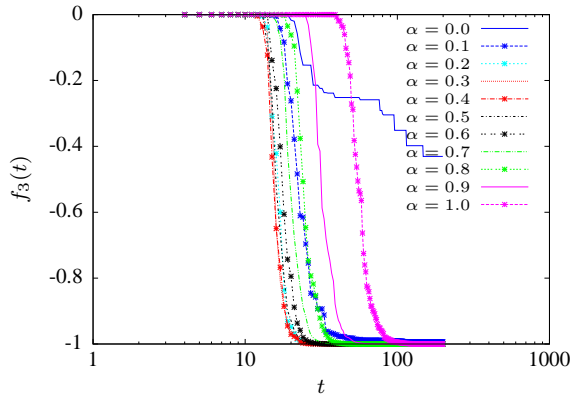
Figure 3: Evolution of the Easom function for \alpha = \{0, \dots, 1\}
