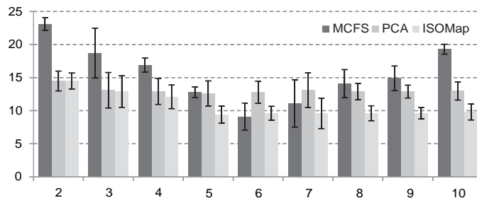
Fig. 3. Classification error according with feature vector optimization methodology and number of extracted features, in percentage.
