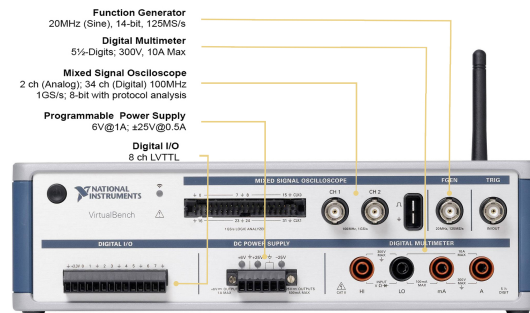
Figura 3.16: Painel frontal VirtualBench VB-8012 [145].
