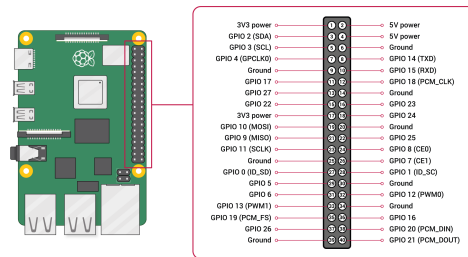
Figura 3.22: GPIO RaspberryPI [148]
