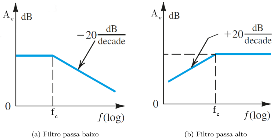
Figura 3.14: Diagramas de Bode [ideal] [144]
