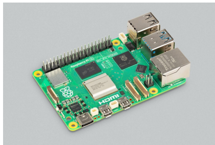
Figura 3.3: Raspberry PI5 [139]
