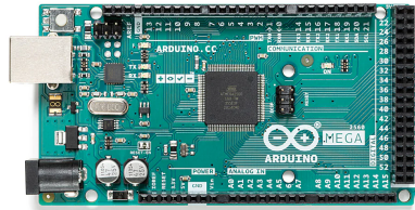
Figura 3.1: Arduino Mega [131]
