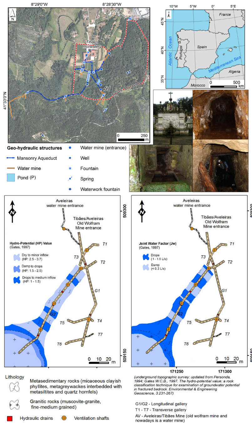
Figure 6: Aveliras mine, S. Martinho de Tibães (Braga, NW Portugal) framework: detailed hydrogeomechanical zoning map for mining hydrogeology and hydrogeotechnics in situ investigations.
