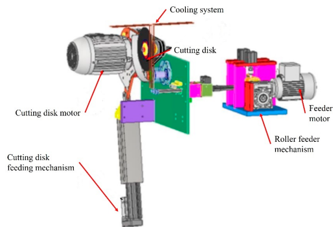
Figure 4. Scheme of the current cutting system.
