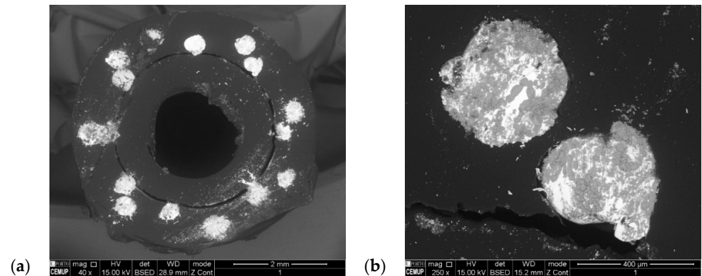
Figure 10. Microscopic images for the braided spiral with diamond disk cut: magnification of 40× (a) and 250× (b).
