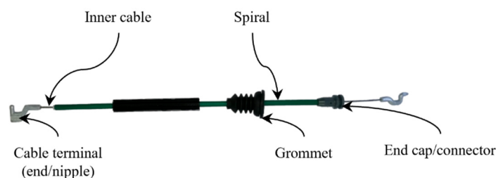
Figure 1. Control cable and its main parts and accessories.
