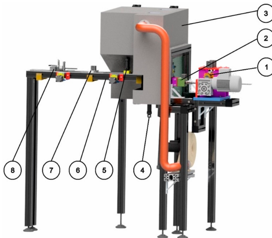
Figure 15. Layout of the cutting mechanism.
