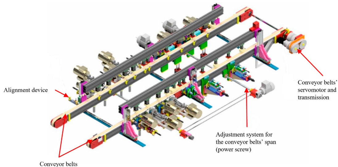
Figure 5. Scheme of the current cleaning/post-processing system.
