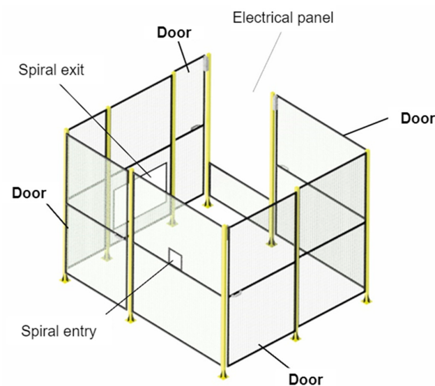
Figure 22. Safety barrier for the machine.
