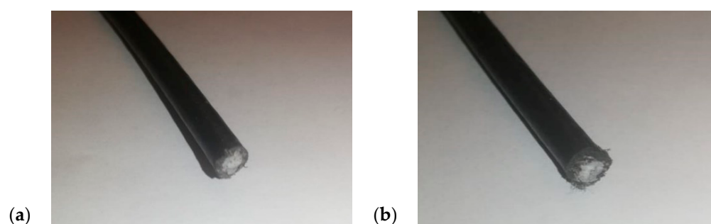
Figure 9. Waterjet cutting with abrasive examples for a push-pull spiral (a) and a braided spiral (b).
