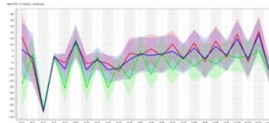
Figure 6: Parallel coordinates plot (Deviation) – teams.
