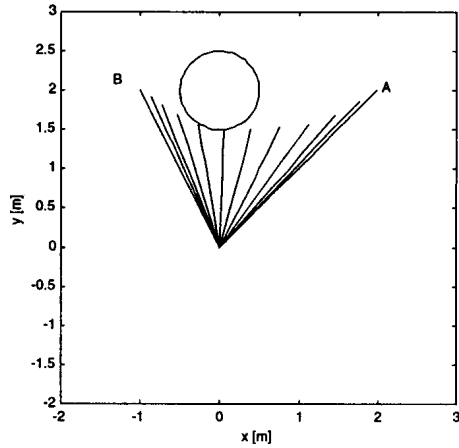
Figure 1: Successive robot configurations for trajectory 1.
