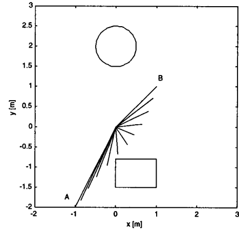
Figure 9: Successive robot configurations.
