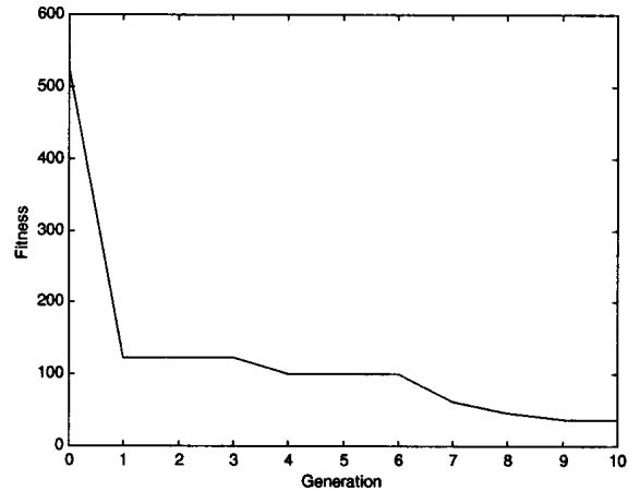
Figure 8: The best individual evolution versus the generation.
