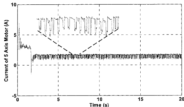
Fig. 11 – Electrical current of the axis motor
