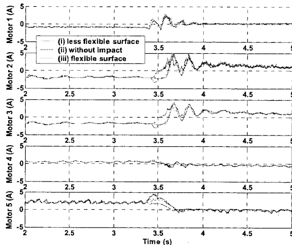
Fig. 14 – Electrical currents of robot axis motors
