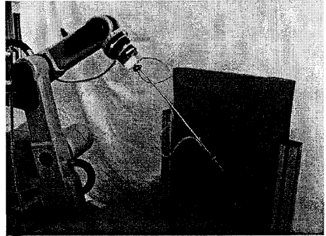
Fig. 12 – Rod impact against a flexible surface
