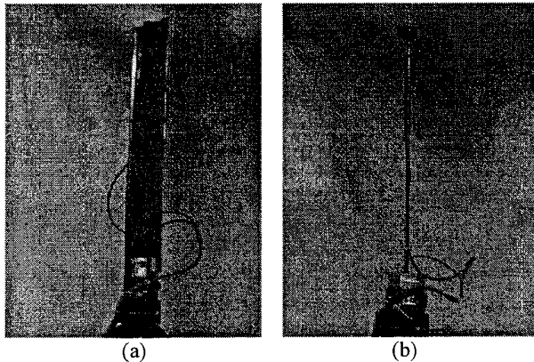
Fig. 8 – Flexible links: (a) Beam and (b) Rod.
