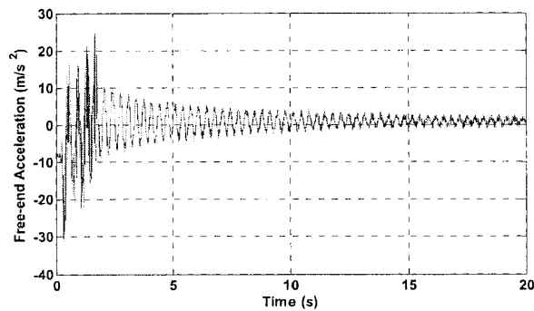
Fig. 9 – Signal of the accelerometer attached at the free-end of the cantilever beam.
