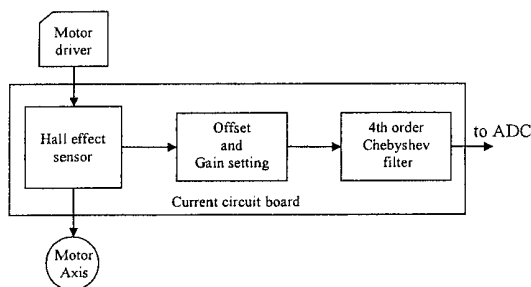
Fig. 3 – Block diagram of current sensor circuit
