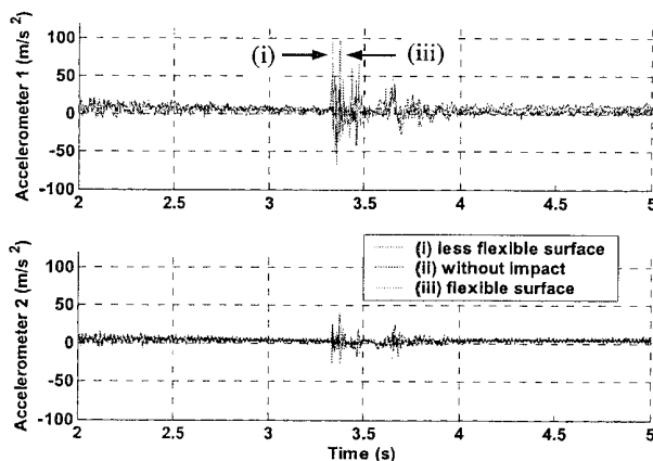
Fig. 15 – Rod accelerations
