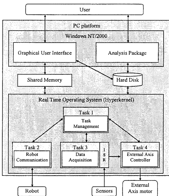
Fig. 4 – Block diagram of software architecture
