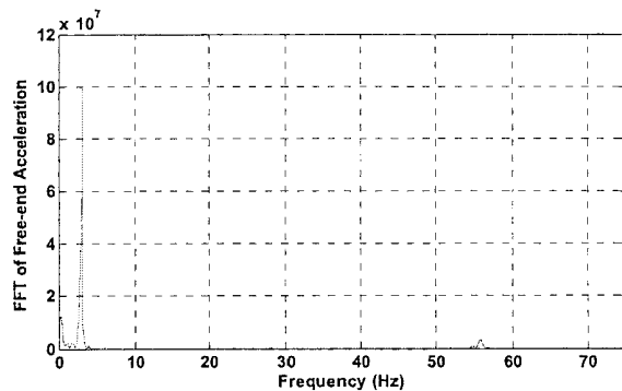
Fig. 10 – FFT of the free-end acceleration
