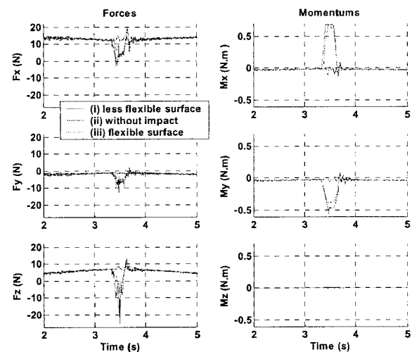
Fig. 13 – Forces and moments due to impact
