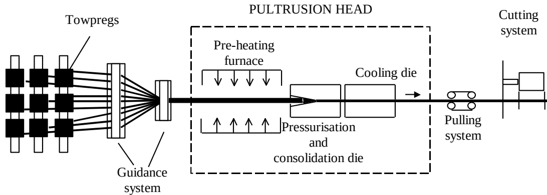
Figure 2. Schematic diagram of the pultrusion line
