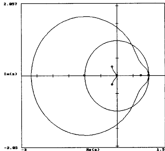
Fig. 5 Z-domain root locus for a mass and control action: D^{1/2}(z) \approx K \left( 1 - \frac{1}{2}z^{-1} - \frac{1}{8}z^{-2} - \frac{1}{16}z^{-3} \right)
