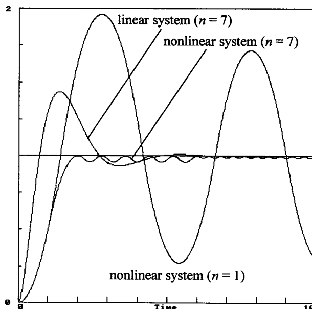
Fig. 12 System response, with relay for a 7-th order series approximation to D^{1/2} .
