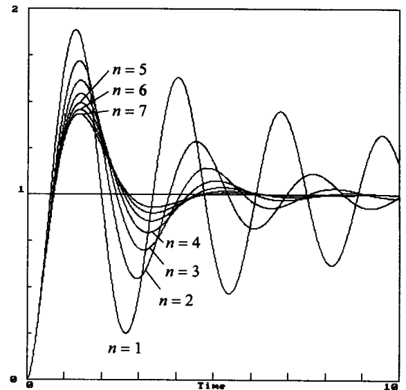
Fig. 8 Linear system response (i.e. without the nonlinear block) for a n -th order series approximation to D^{1/2} .
