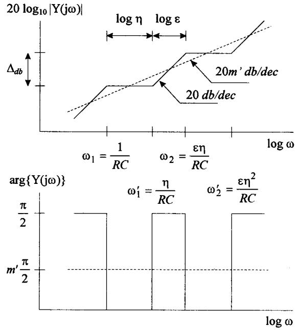
Fig. 2 Bode diagrams of amplitude and phase of Y(jω).
