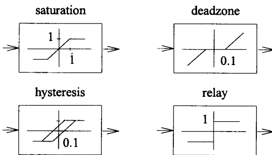
Fig. 7 Nonlinear phenomena at the actuator: saturation, deadzone, hysteresis and relay.
