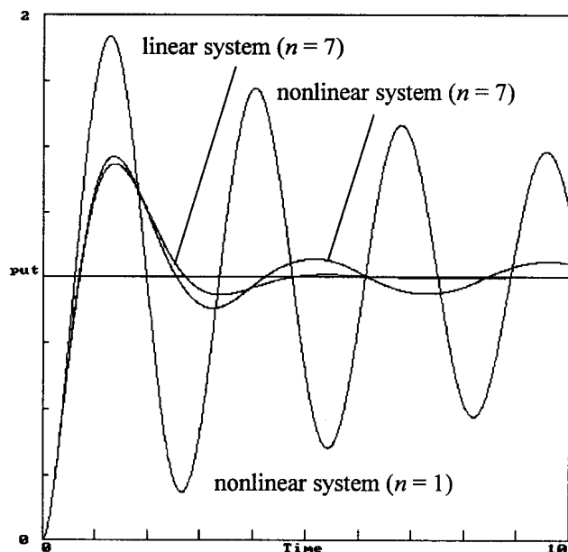
Fig. 11 System response, with hysteresis for a 7-th order series approximation to D^{1/2} .
