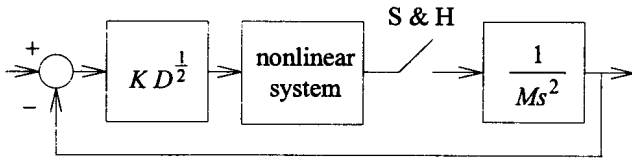
Fig. 6 D^{1/2} controller for a system with a mass and a nonlinear actuator.
