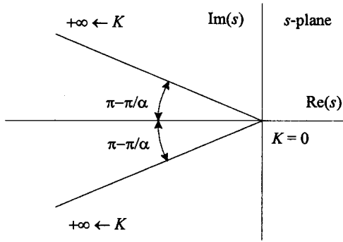
Fig. 4 Root locus for a feedback control system of fractional order 1 < \alpha < 2 .
