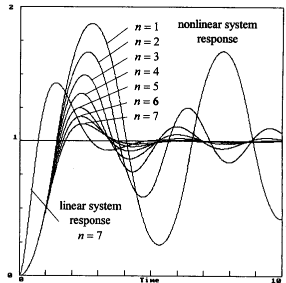
Fig. 9 System response, with saturation for a n -th order series approximation to D^{1/2} .
