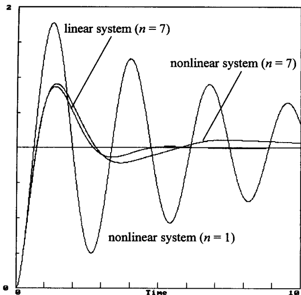
Fig. 10 System response, with deadzone for a 7-th order series approximation to D^{1/2} .
