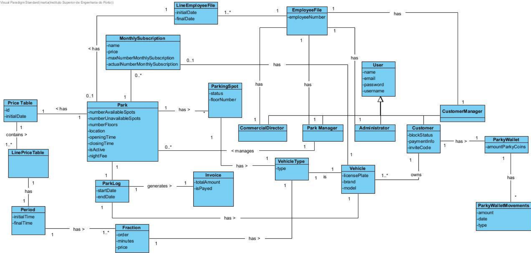
Figure 6 - Domain Model
