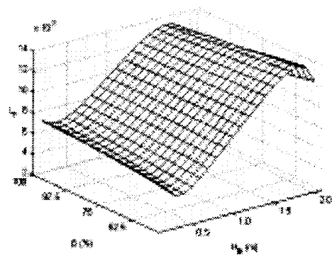
Fig. 15. Plot of L_F vs. (\beta, H_B) for F_C = 0.01 m, L_S = 1 m, WG.
