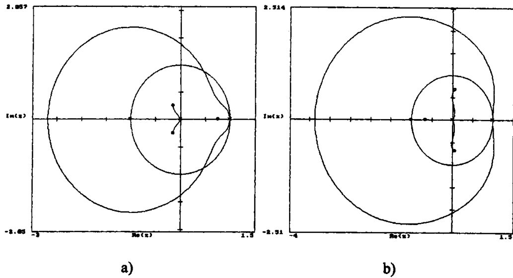
FIGURE 5 Z-domain root locus for a mass and fractional control actions based on a 3-th order series approximation: a) D^{1/2}(z) \approx K(1 - 1/2 z^{-1} - 1/8 z^{-2} - 1/16 z^{-3}) b) I^{1/2}(z) \approx K(1 + 1/2 z^{-1} + 3/8 z^{-2} + 5/16 z^{-3}) .
