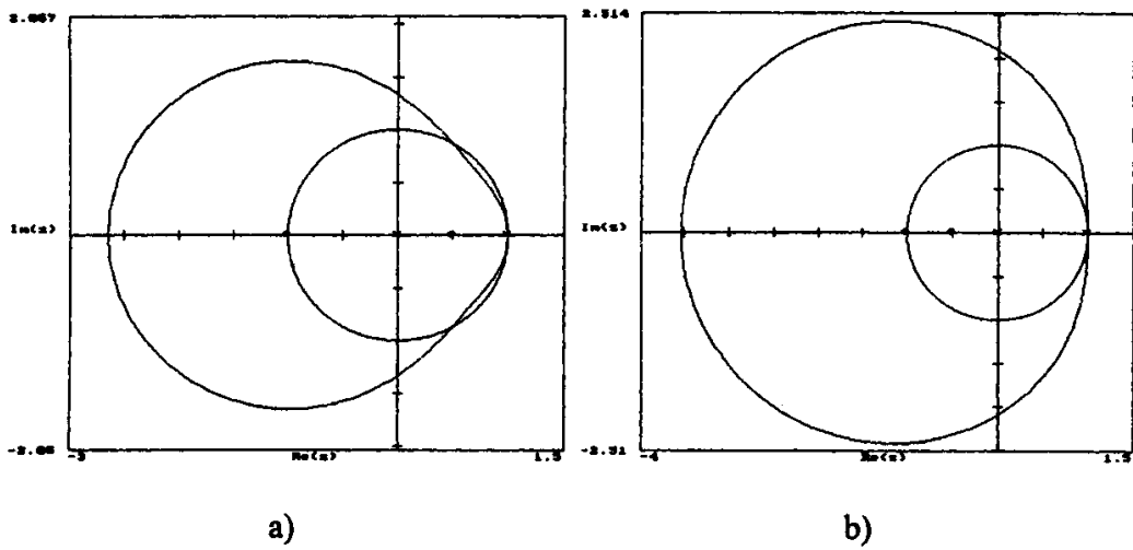
FIGURE 6 Z-domain root locus for a mass and fractional control actions based on a linear interpolation: a) D^{1/2} b) I^{1/2} .
