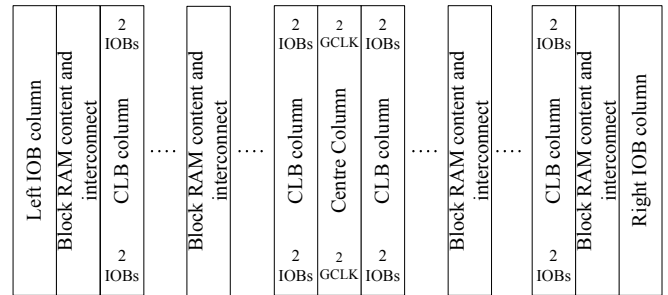
Fig. 2: Configuration memory organization.
