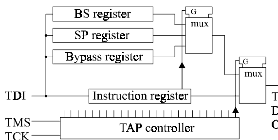
Figure 1: The group of test data registers after implementing the SELPIN optional instruction.
