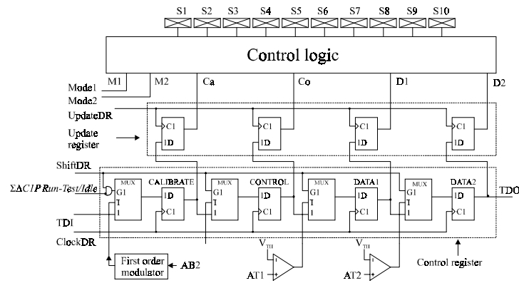
Figure 9: TBIC - Example implementation of the control structure supporting the \Sigma AC1P instruction.
