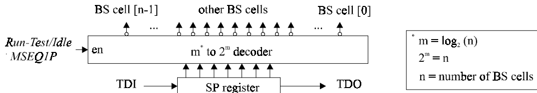
Figure 8: Decoder ( m to 2^m ) that identifies the BS cell associated with the selected pin.
