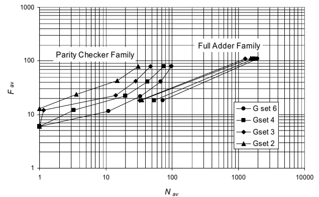
Fig. 4. F_{av} versus N_{av} for the parity checker and the full adder circuits families and the Gsets under evaluation.
