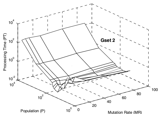
Fig. 5. PT versus (P, MR) with CR = 95\% using Gset 2 for the 2-to-1 Multiplexer
