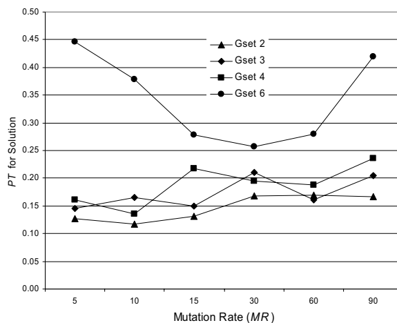
Fig. 6. PT for solution versus MR , with CR = 95\% and P = 70 , for the 2-to-1 Multiplexer
