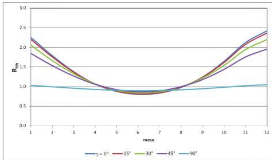
Figure 6.1.5 - Influence of azimuth variation on southern orientation ( \gamma = 0^\circ ) on the irradiation of a fixed 40^\circ inclined surface
