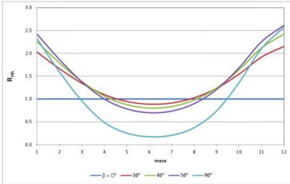
Figure 6.1.4 - Influence of the inclination variation on a monthly basis for a fixed orientation collector south \gamma = 0 at the latitude of \phi = 40^\circ
