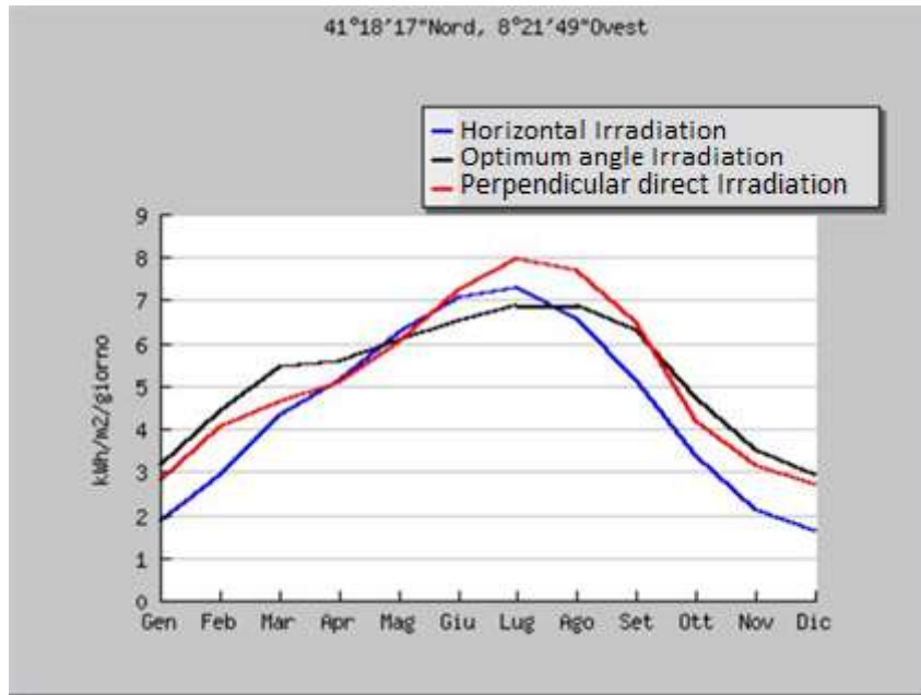
Figura 6.1.1.2 - Available irradiation comparison
