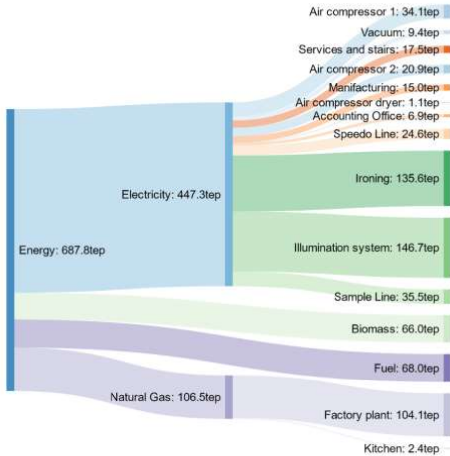
Figure 5.7.3 – Sankey's diagram
