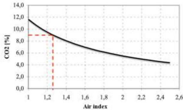
Figure 4.5.5.5 - Relationship between CO 2 in fumes and air index
