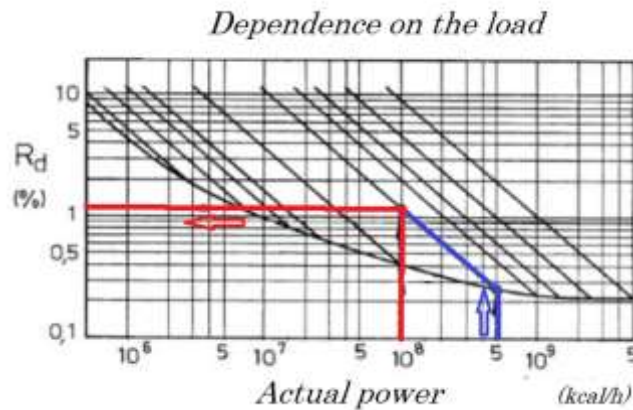
Figure 4.5.5.2 - Influence of load according to the plant's potential and irradiation losses
