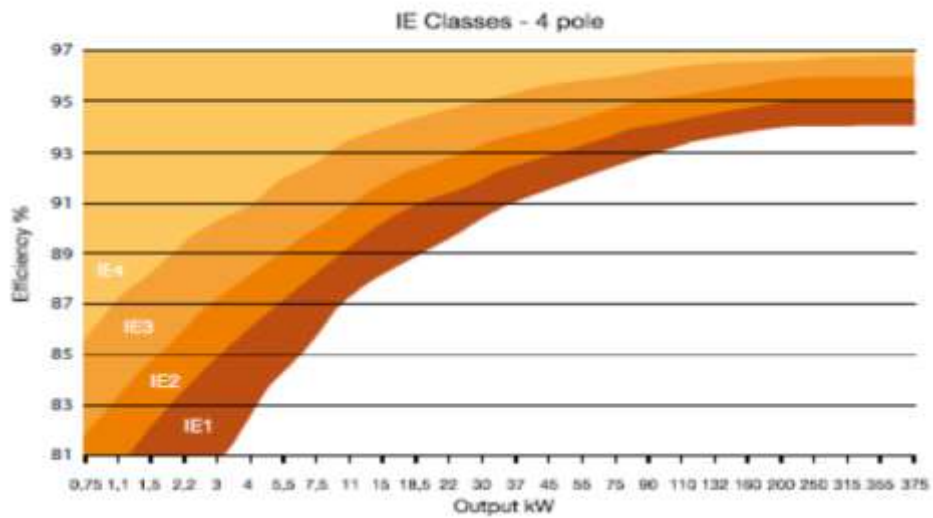
Comparison Table of Performance Bands according to CEMEP
