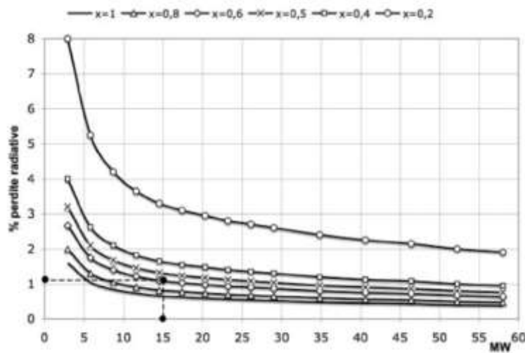
Figure 4.5.5.3 – Graph to find radiative losses %
