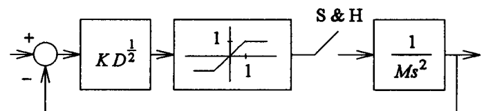
Figure 8: FDI control system of a mass system with actuator saturation.
