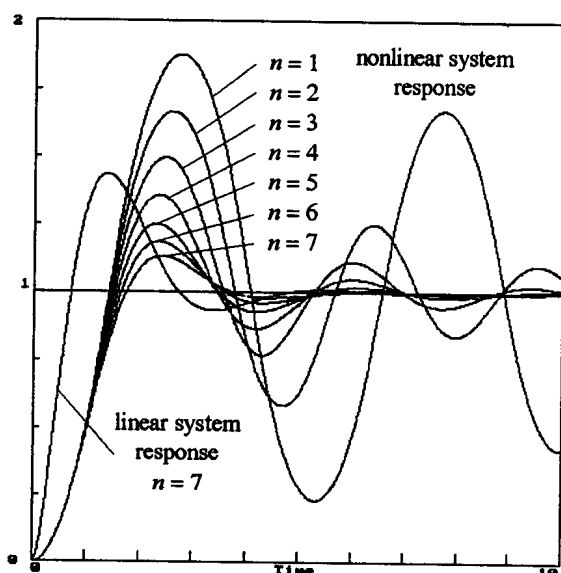
Figure 10: System response, with saturation, for K = 10 M and a n -th order series approximation to D^{1/2} .
