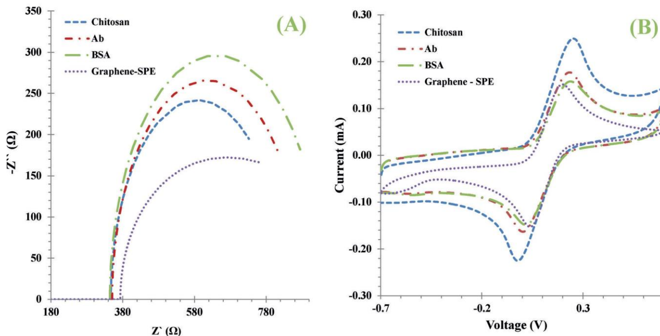
Fig. 2. EIS spectra of each stage of the assembly of the immunosensor (A) and CV data taken at each stage (B). (A) Nyquist plots of BSA/anti-hCG/CS/graphene-SPE sensor, obtained in 5.0 mM [\text{Fe}(\text{CN})_6]^{3-/4-} PBS buffer pH 7.4. (B) CV record after modification of chitosan/AuNPs/graphene-SPE with antibody and BSA.
