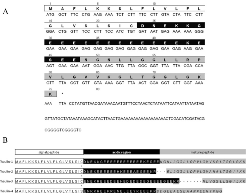
Fig. 2. (A) Nucleic acid and deduced amino acid sequence of cDNA encoding thaulin-1 from the skin of P. thaul . Signal peptide, acidic region and mature peptide are signaled in boxed white, black and gray letters respectively and stop codon is indicated with an asterisk. (B) Alignment of the deduced amino acid sequences of the precursors of thaulin peptides. Preproregions (signal peptide and acidic region boxed white and black respectively) and variable domain (boxed gray) that correspond to mature peptide are signaled. Cys indicating the end of the signal peptide are indicated with an asterisk. Processing sites Lys-Arg present in the acidic region are underlined. Gaps (-) have been introduced to maximize sequence similarities.
