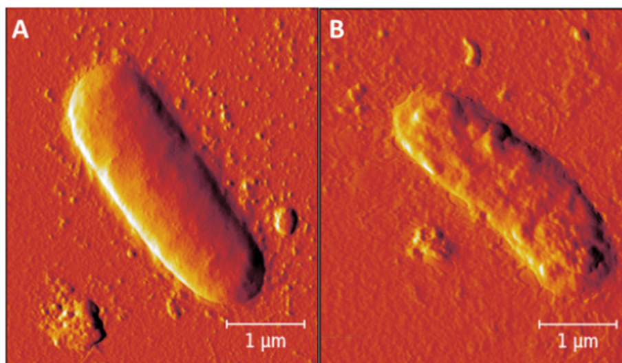
Fig. 4. Representative AFM image of the antimicrobial effect of thaulin-1 on E. coli ATCC 25922: (A) untreated; (B) after 24 h of thaulin-1 treatment at the MIC.
