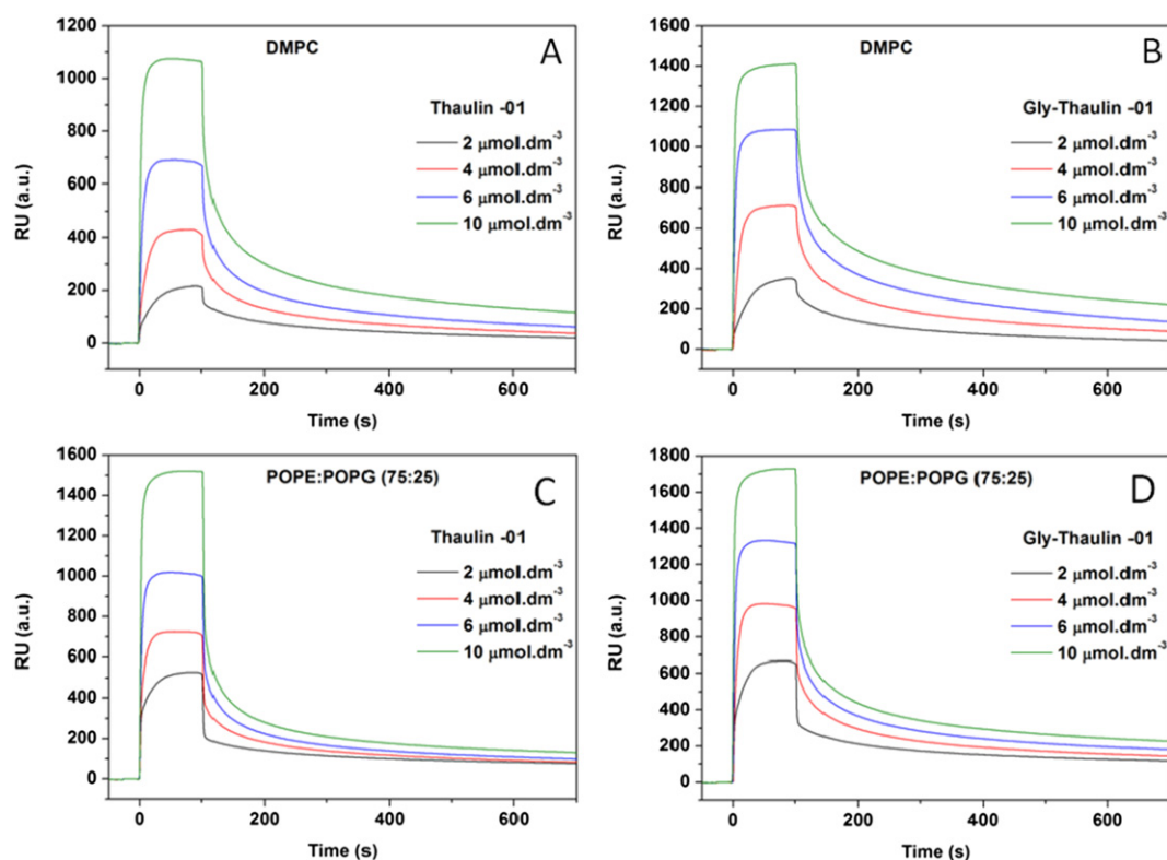
Fig. 5. Representative Surface Plasmon Resonance sensograms obtained for thaulin-1 and Gly-thaulin-1 binding to mimetic membrane models. (A) and (B) DMPC supported unilamellar bilayers. (C) and (D) POPE:POPG (75:25) supported unilamellar bilayers.
