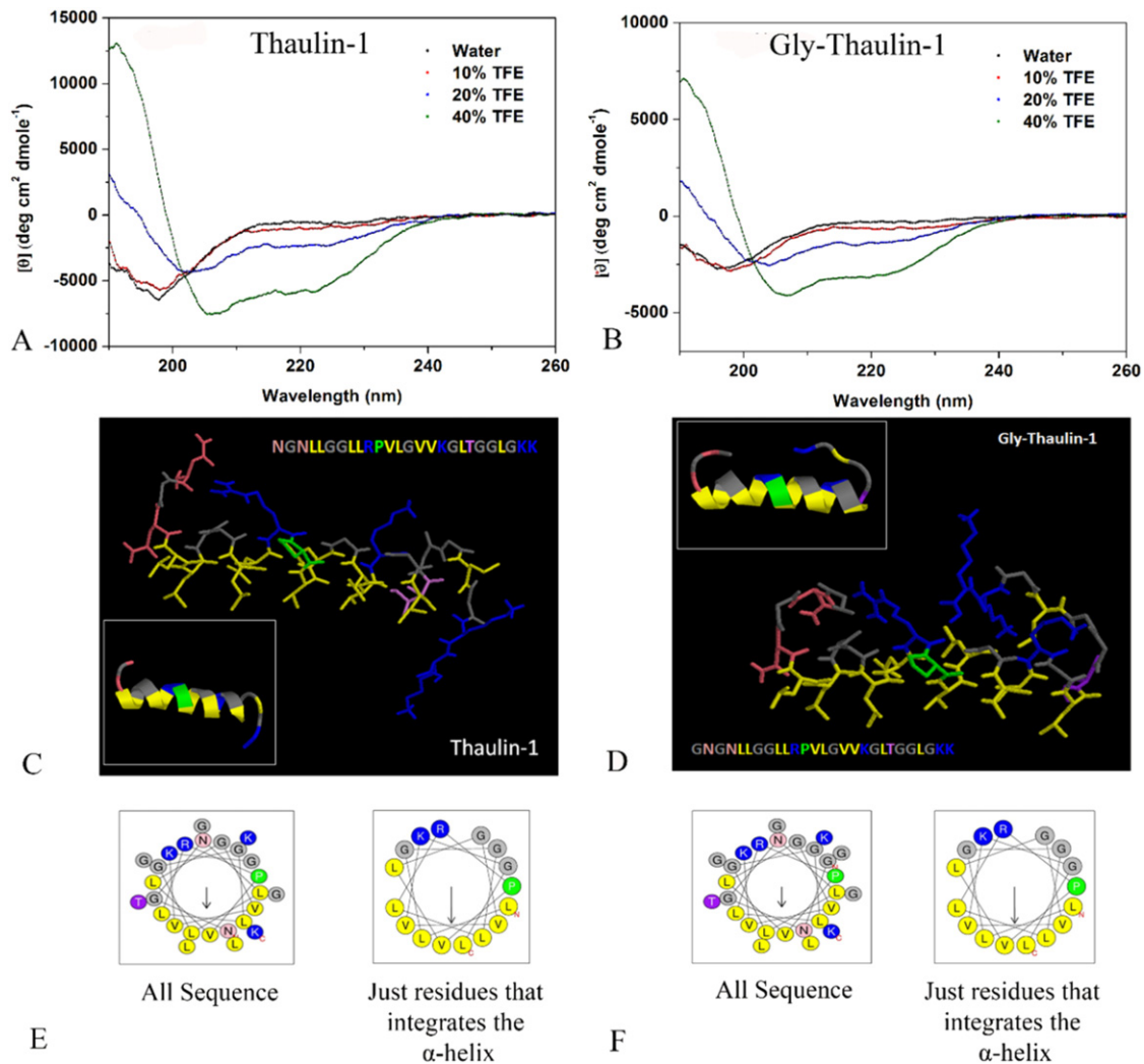
Fig. 3. Graphical analysis of thaulin-1 and Gly-thaulin-1 peptide structures. Circular dichroism of peptides (A) thaulin-1 and (B) Gly-thaulin-1 in aqueous (black) and 10, 20 and 40% of 2,2,2-trifluoroethanol (TFE) solutions (red, blue and green respectively). (C) thaulin-1 and (D) Gly-thaulin-1 3D structure prediction. Schiffer and Edmundson wheel projection diagrams of complete and \alpha -helix fragment of (E) thaulin-1 and (F) Gly-thaulin-1 sequences. Amino acid colour code: yellow = unpolar/hydrophobic (Leu, Val), gray = Gly, blue = basic (Lys, Arg), purple = polar without charge (Thr), pink = polar without charge (Asn), green = Pro.
