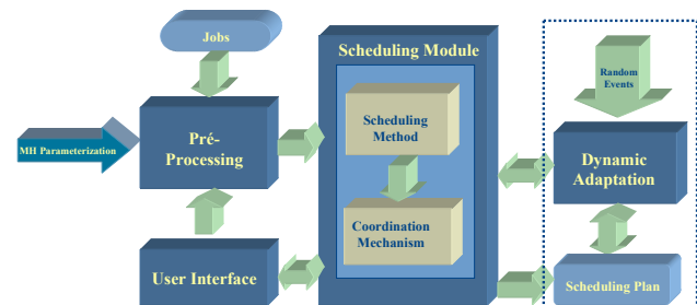
Figure 1. AutoDynAgents System Architecture
