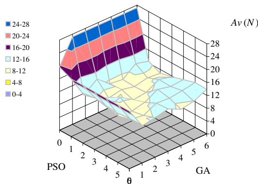
Figure 7: Av(N) for the M2 - 1 circuit using Gset 4
