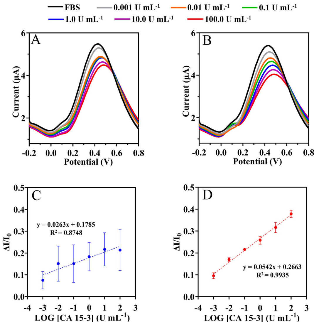
Fig. 8 SWV measurements of NIPs (A) and MIPs (B) based biosensor and the corresponding calibration curves (C) and (D) respectively, in 5 mmol \text{L}^{-1} [\text{Fe}(\text{CN})_6]^{3-} and 5 mmol \text{L}^{-1} [\text{Fe}(\text{CN})_6]^{4-} by increasing CA 15-3 protein in the fetal bovine serum.
