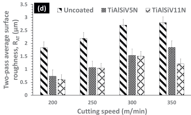
Fig. 5. Variation of surface roughness with cutting speed for (a) \text{Al}_2\text{O}_3/\text{SiC} uncoated, (b) TiAlSiV5N coated, and (c) TiAlSiV11N coated tools for two passes. (d) Variation of two-pass average surface roughness with cutting speed.
