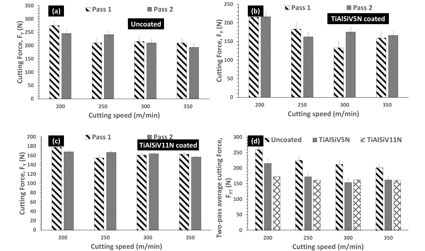
Fig. 3. Variation of cutting force with cutting speed for (a) \text{Al}_2\text{O}_3/\text{SiC} uncoated, (b) TiAlSiV5N coated, and (c) TiAlSiV11N coated tools for two passes. (d) Variation of two-pass average cutting force with cutting speed.
