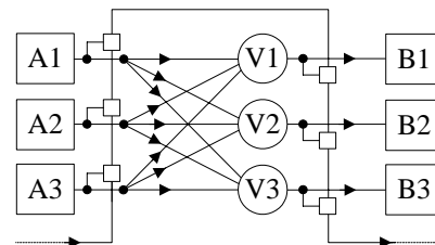
Fig. 2. Example of a T-TMR implementation with a scan chain
