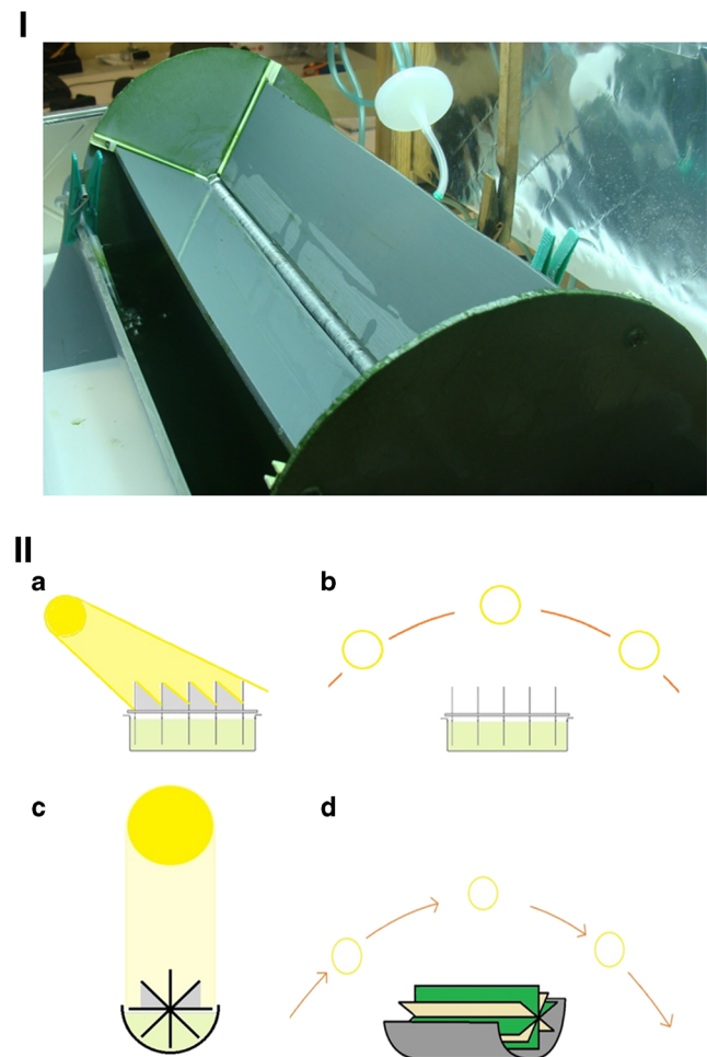
Fig. 4 (I) Rotating plate photobioreactor (RFPPB) projected and tested in this work. (II) Schematic representation of solar light incidence over the disks of a RBC-type photobioreactor during part of a day (a); variation of solar position over an RBC along 1 day (b); schematic representation of the new RFPPB photobioreactor and solar radiation incidence over the plates of the RFPPB at noon (c); solar incidence variation over the RFPPB during 1 day (d)
