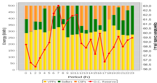
Figure 4. Operation costs and dispatched energy related to the reserve product, for the 24 periods of the day.
