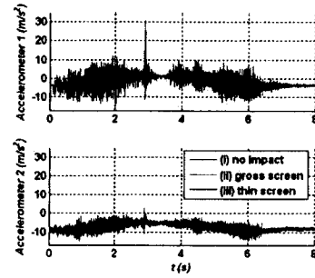
Fig. 3.5 Rod accelerations.
