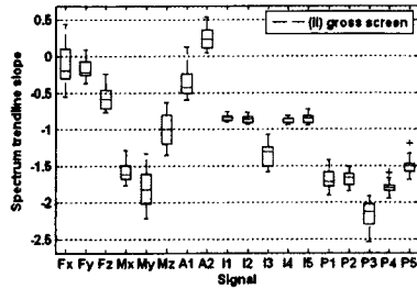
Fig. 3.14 Statistics of spectrum trendlines slopes for the gross screen.
