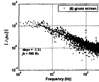
Fig. 3.9 Spectrum of the axis 3 motor current.
