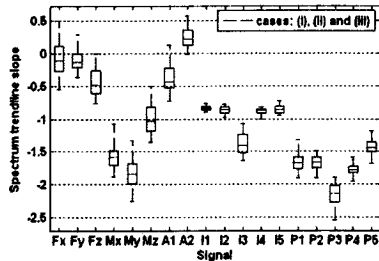
Fig. 3.15 Statistics of spectrum trendlines slopes for all the cases (i, ii, iii).
