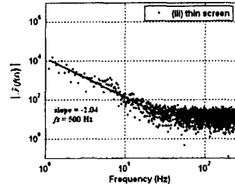
Fig. 3.8 Spectrum of the axis 3 position.
