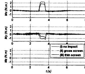
Fig. 3.4 Torques at the gripper sensor.
