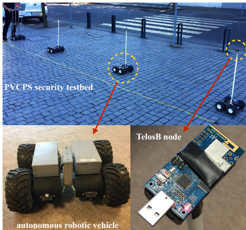
Figure 1: The CoopKey testbed for PVCPS security.
