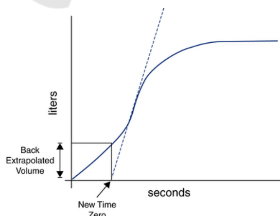
Figure 1: Volume-time curve showing the calculation of the Back Extrapolated Volume.
