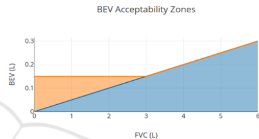
Figure 8: In orange, the acceptable BEV ranges using the ATS guidelines; in blue, the ranges using the implemented algorithm (The ATS ranges overlap with the algorithm's ranges).
