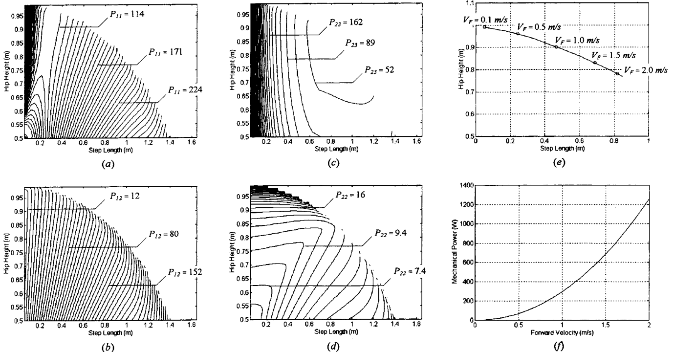
Fig. 6 - Contour plots of the absolute power P_m at the individual joints: (a) stance ankle, (b) stance knee, (c) swing hip, (d) swing knee; (e) Optimal (L_S, H_H) locus vs forward velocity V_F , (f) Absolute power vs forward velocity V_F .
