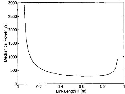
Fig. 11 - Performance index P_m vs link length l_1 .
