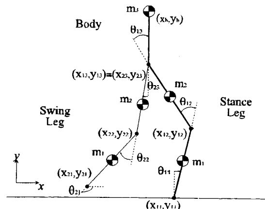
Fig. 1 - Planar biped model.
